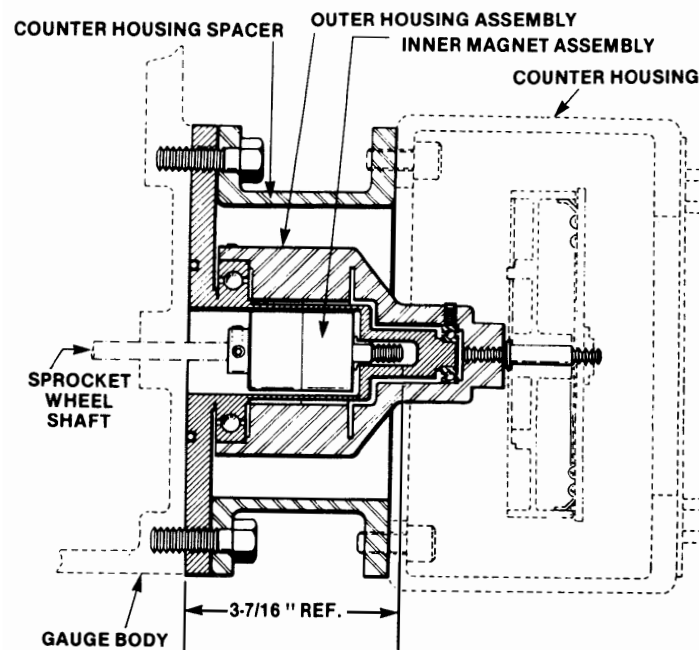
Magnetic Drive Motor Option
